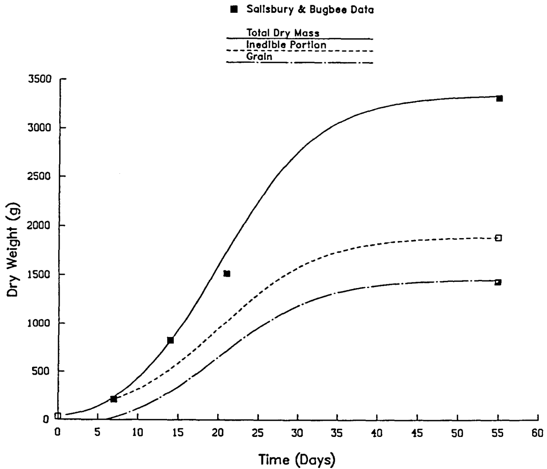
Fig. 2. Wheat growth in 1 m 2 from both actual data and the plant-growth submodel used in the BLSS Simulation Model. Growing conditions in the model were constant light, 1000 μl/l CO 2 , and 4.0 mM NO 3 - .
